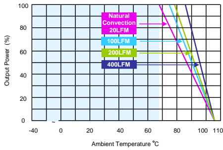
AER50-72S24, AER50-110S12, AER50-110S24 Derating Curve without Heatsink
