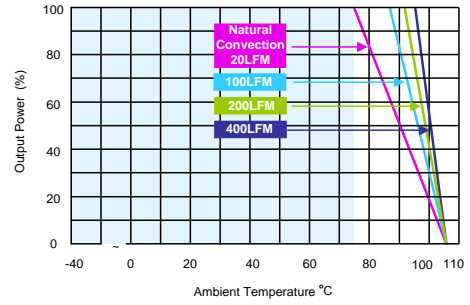
AER50-72S12, AER50-72S15, AER50-110S15 Derating Curve with Heatsink
