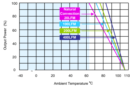
AER50-72S05, AER50-110S05 Derating Curve without Heatsink
