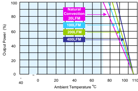
AER50-72S12, AER50-72S15, AER50-110S15 Derating Curve without Heatsink
