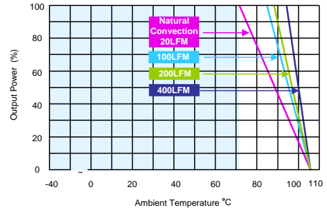
AER50-72S24, AER50-110S12, AER50-110S24 Derating Curve with Heatsink
