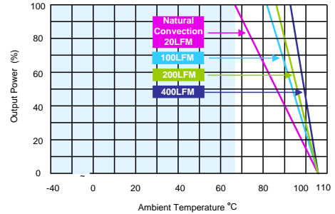
AER50-72S05, AER50-110S05 Derating Curve with Heatsink
